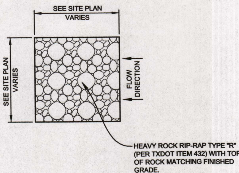
VELOCITY CONTROL DETAIL N.T.S.
