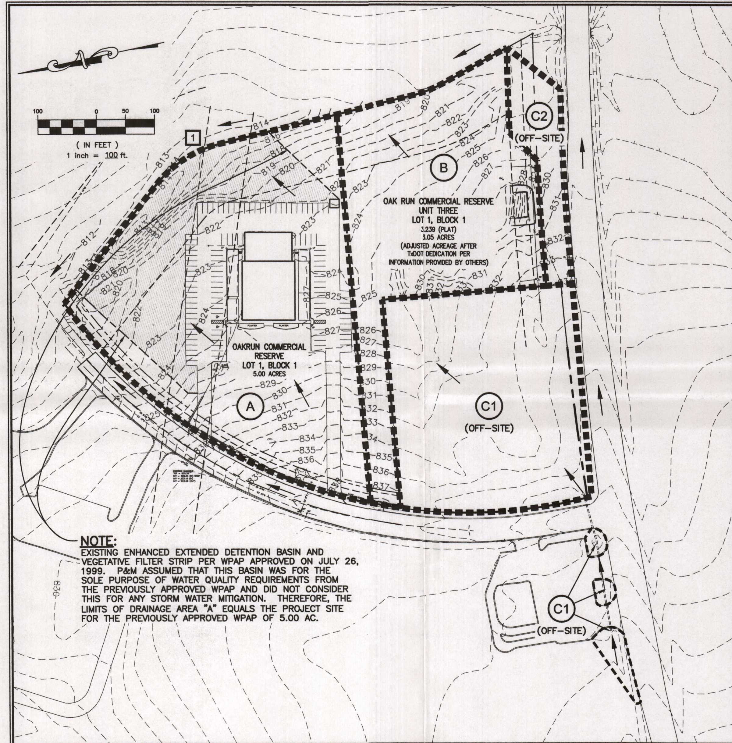
EXISTING DRAINAGE CONDITIONS
